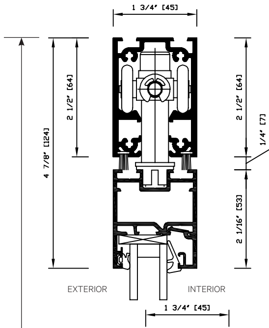
Detail 1.1 Head Jamb
