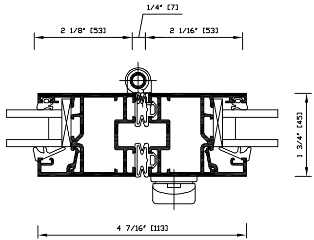
Detail 7.0 & 7R.0 Folding panel with locking (Handle may be on left panel.)
