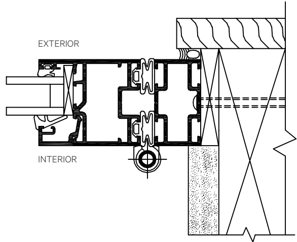
Inward Opening Panel Hinged At Right Side Jamb
