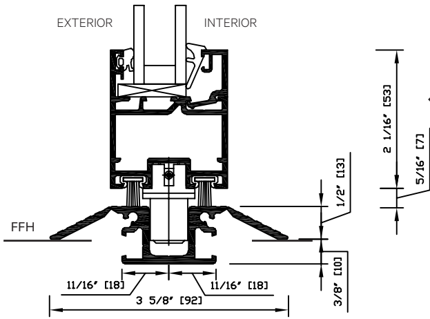
◀ Detail 2.0 Standard Sill (Limited water rating against wind driven rain with weepholes by others.)
