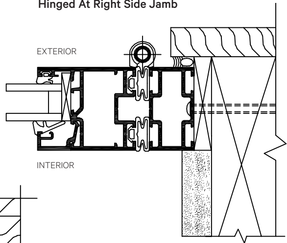
Outward Opening Panel Hinged At Right Side Jamb
