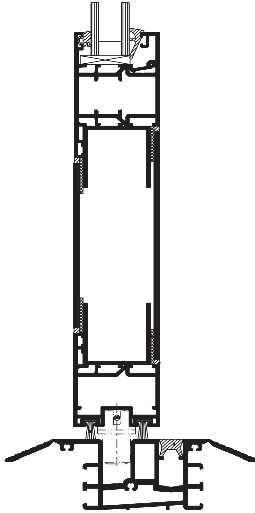
Typical Kickplate
