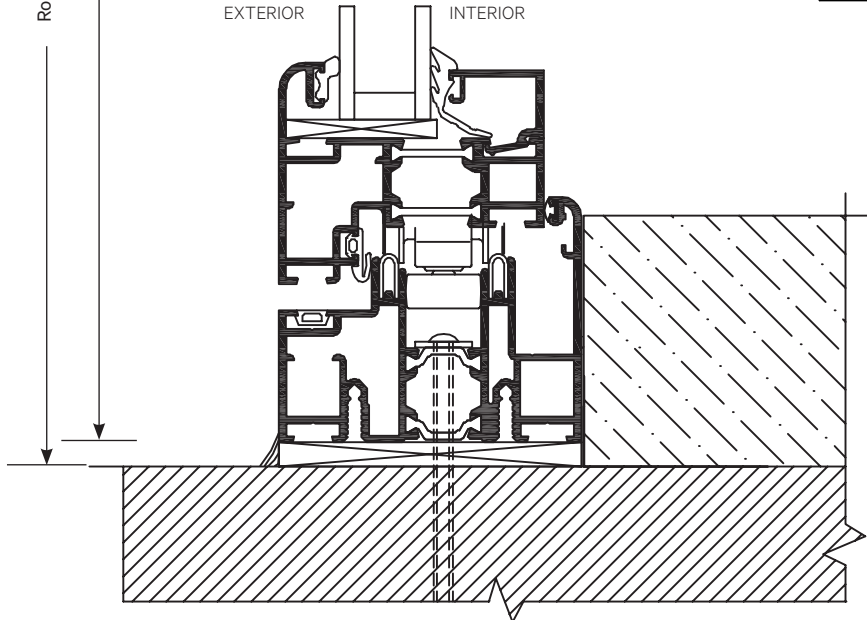
Higher Weather Performance Sill (Raised Sill) Installation
