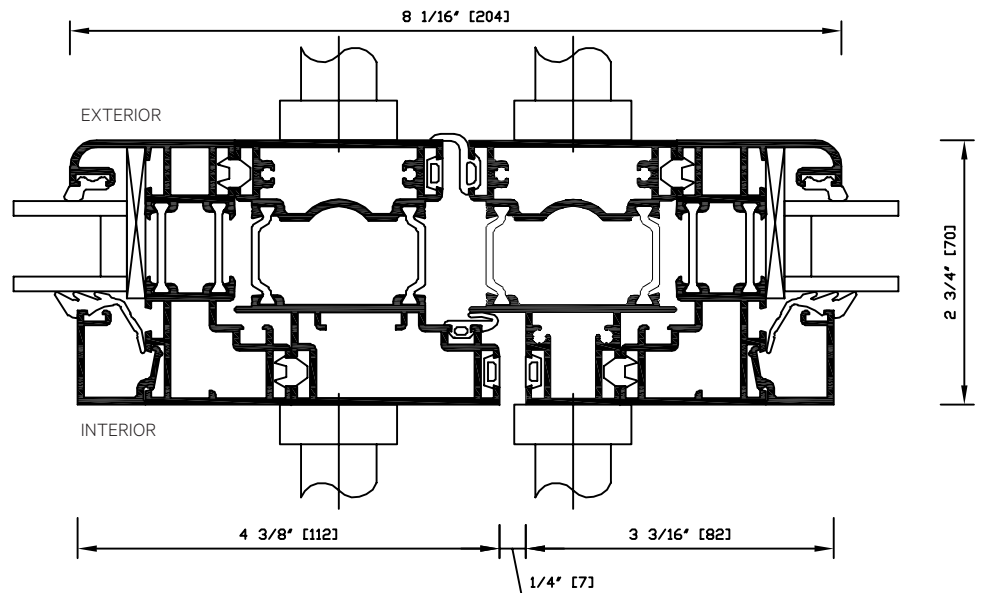
Detail 8.0 Two swing panels with locking: left panel opening first
