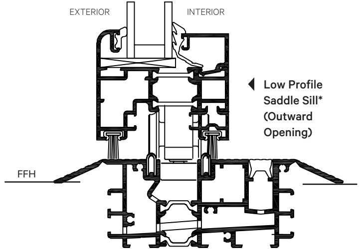
◀ Flush Sill (Inward Opening) (No rating against wind driven rain.)
