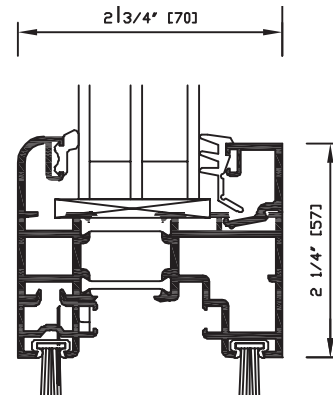
Typical Glass Stop Profile with Triple Glazing
