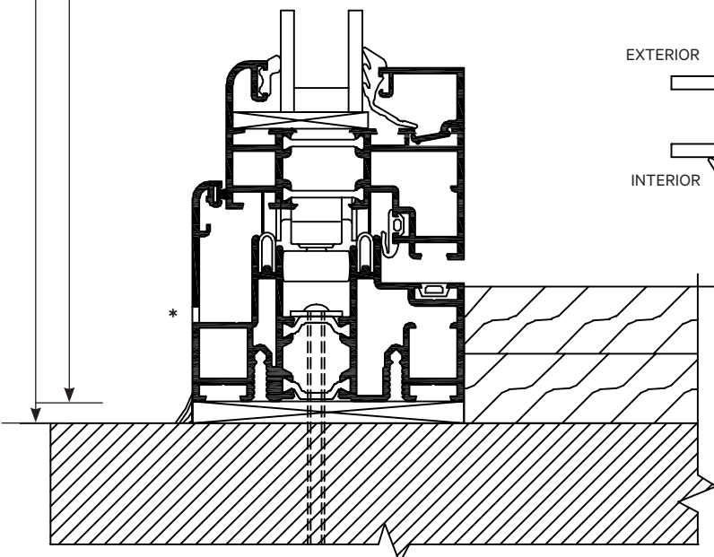
Standard Higher Weather Performance Sill (Raised Sill)
