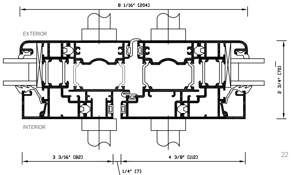
Detail 8R.0 Two swing panels with locking: right panel opening first
